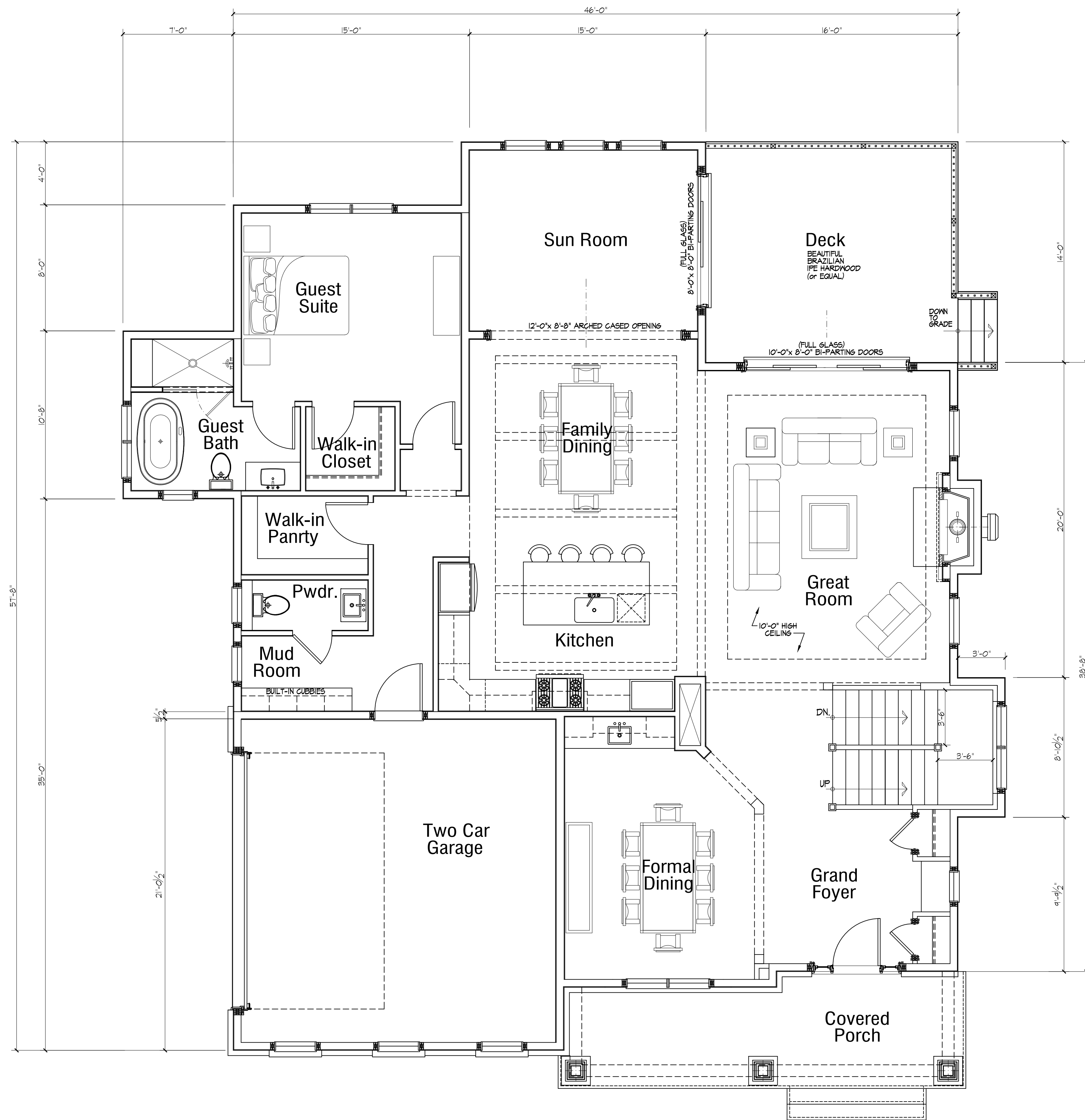
First Floor Plan 1,945 Sq. Ft. - Living 155 Sq. Ft. - Front Porch 224 Sq. Ft. - Deck 432 Sq. Ft. - Garage
